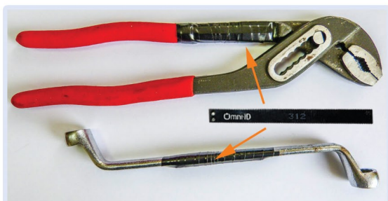
Permanent marking with RFID UHF tag
